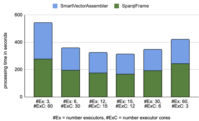
Figure 9: Spark setup vs Processing time
