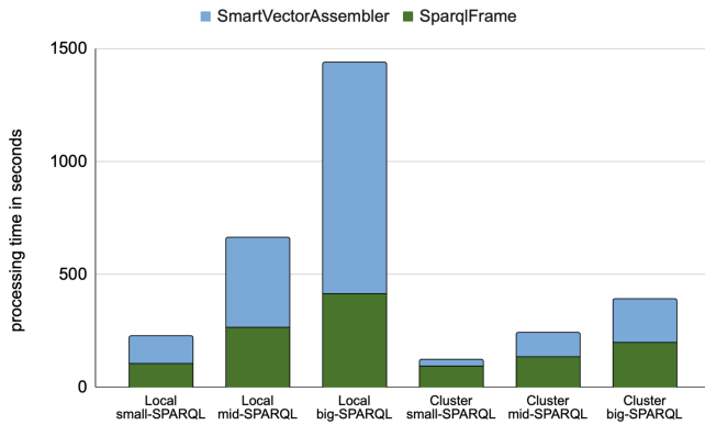
Figure 7: SPARQL complexity vs processing time
